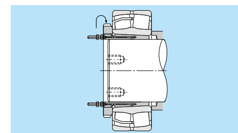
Fig. 15.39 Disassembly using hydraulic withdrawal sleeve
