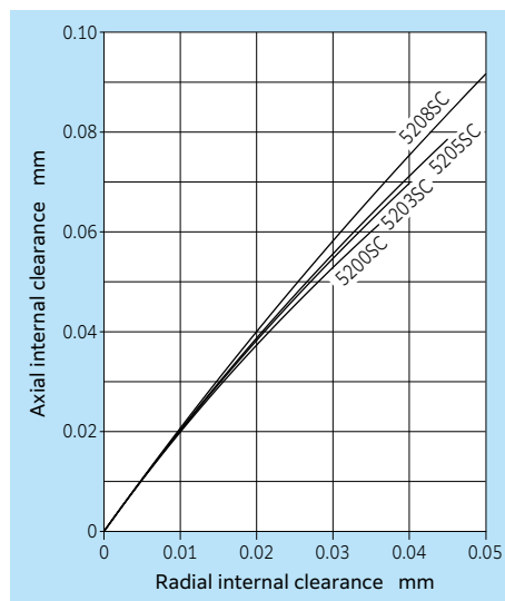
Fig. 17.1.8 Series 52SC radial internal/axial internal clearances
