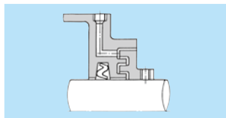
Fig. 8 Combination seal
