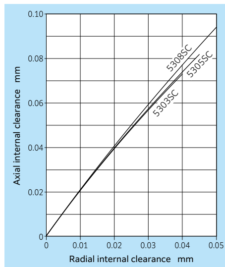
Fig. 17.1.9 Series 53SC radial internal/axial internal clearances
