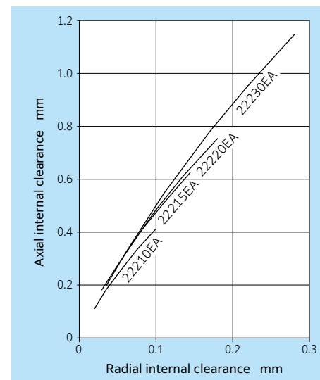
Fig. 17.1.10 Series 222 radial internal/axial internal clearances
