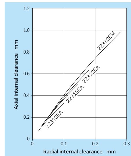
Fig. 17.1.11 Series 223 radial internal/axial internal clearances
