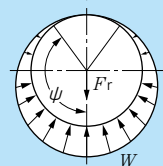
Fig. 3.12 0.5 < \varepsilon < 1 90^\circ < \psi < 180^\circ Radial preload state, or large axial load
