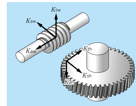
Fig. 4.7 Worm gears
