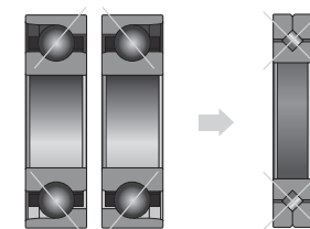
Traditional Ball bearing Cross Roller Bearing
